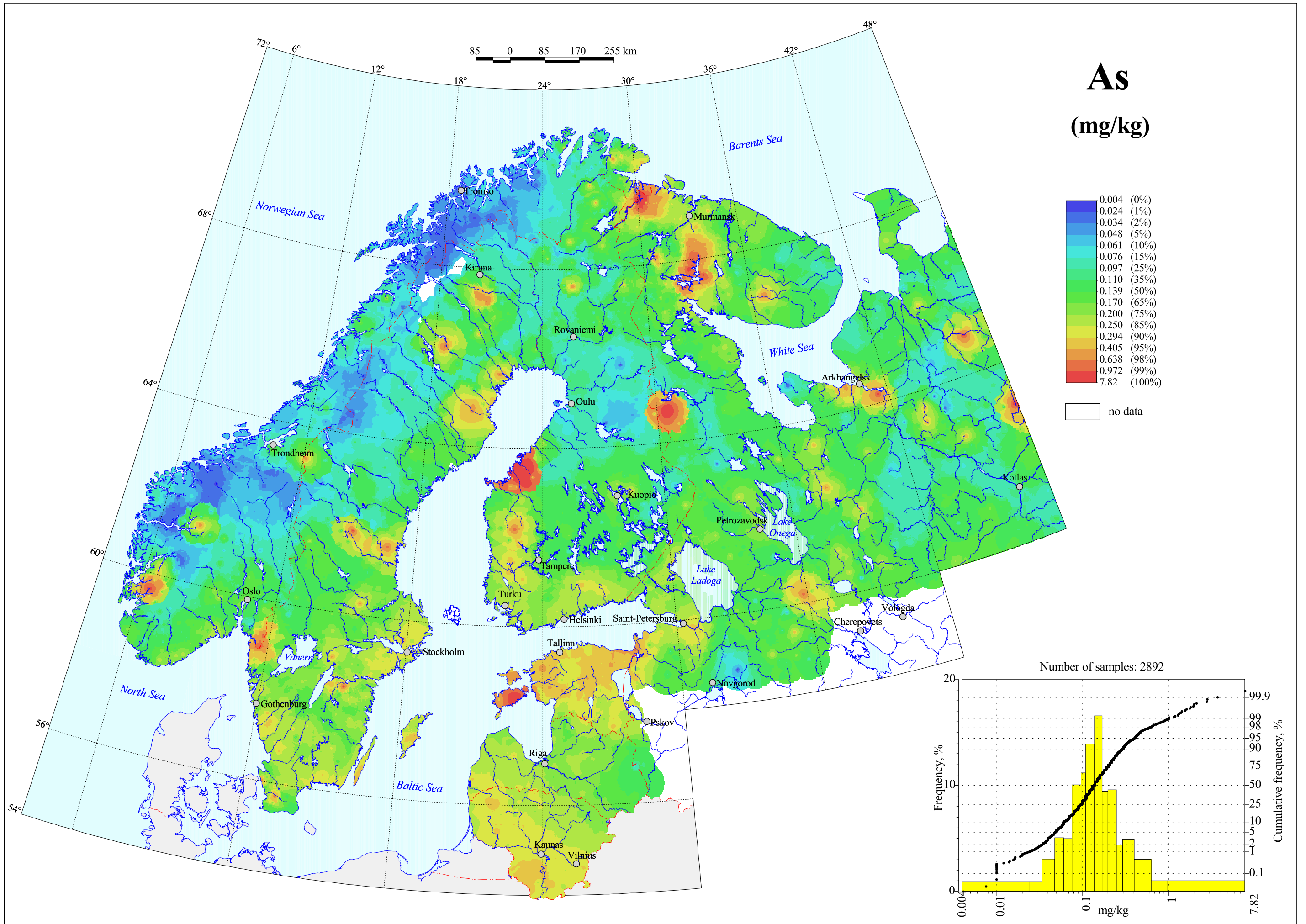
Arsenic in Terrestrial Moss, Total Content
